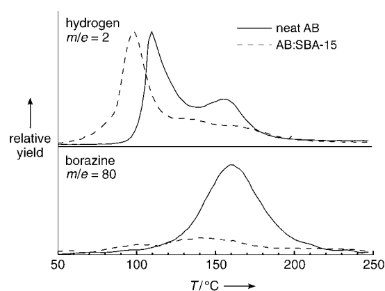
Figure 2. TPD/MS ( 1^\circ\text{C min}^{-1} ) of volatile products generated by heating neat ammonia borane (solid line) and AB:SBA-15 (dashed line); m/e=2 ( H_2 ) and m/e=80 (borazine, c\text{-NHBH}_3 ). The value m/e=2 ( H_2 ) is normalized to the area under the curve for neat ammonia borane (solid line). The corresponding scalar was used to normalize the m/e=80 borazine data for AB:SBA-15.
